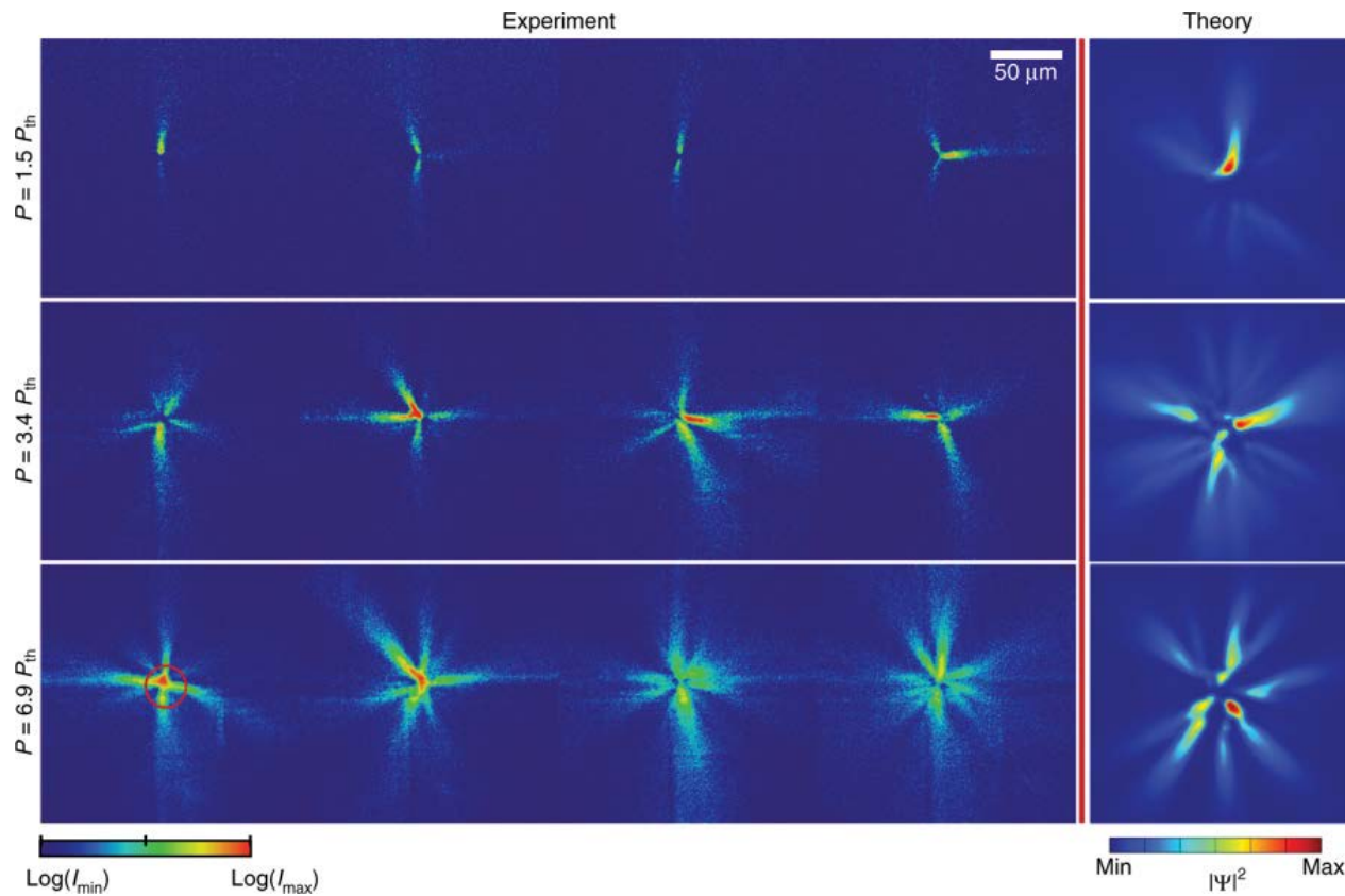
Single-shot condensation of polaritons. Theory (on the right) shows remarkable agreement with experiment (left).
