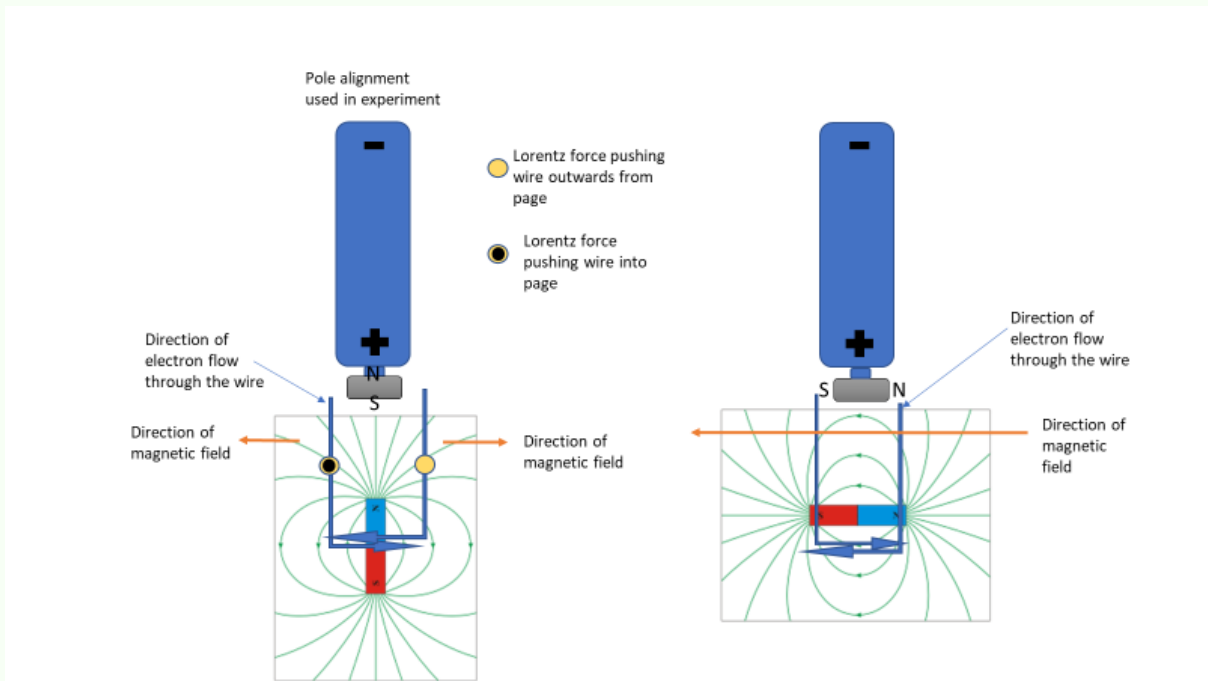
Figure 2. Operation of spinning wire showing direction of electron flow through the wire, the magnetic field and effect of Lorentz Force.
